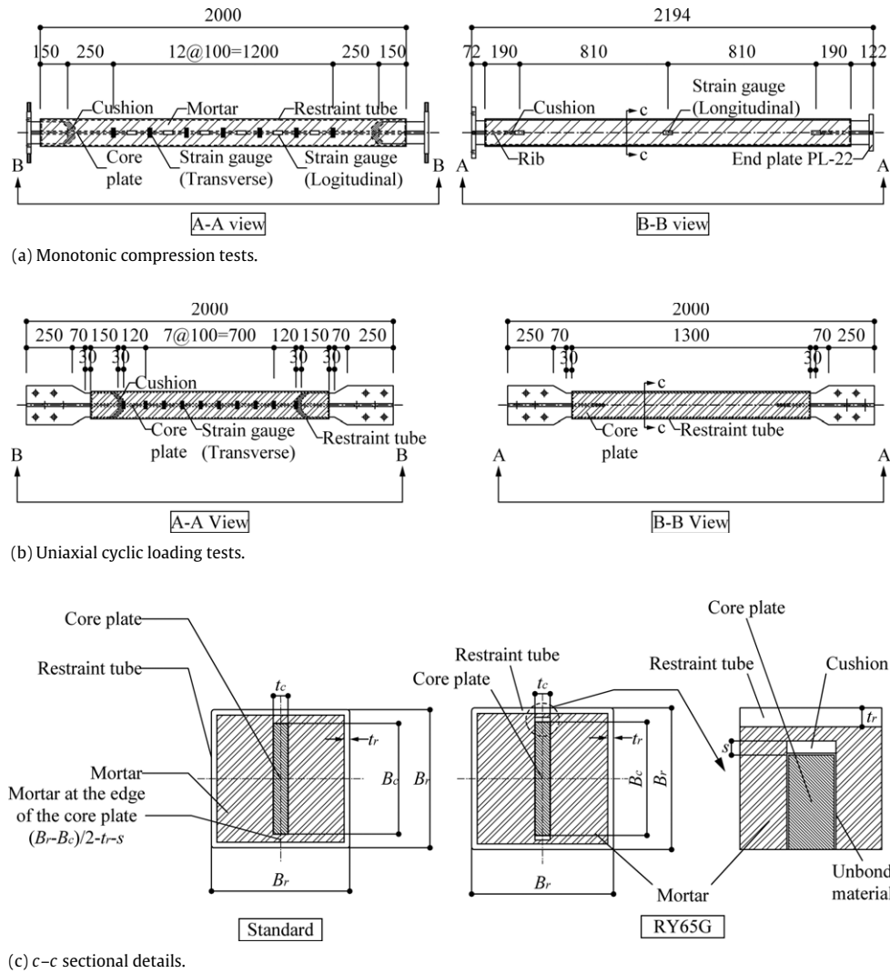
Fig. 3. Specimens for monotonic compression tests and uniaxial cyclic loading tests.
