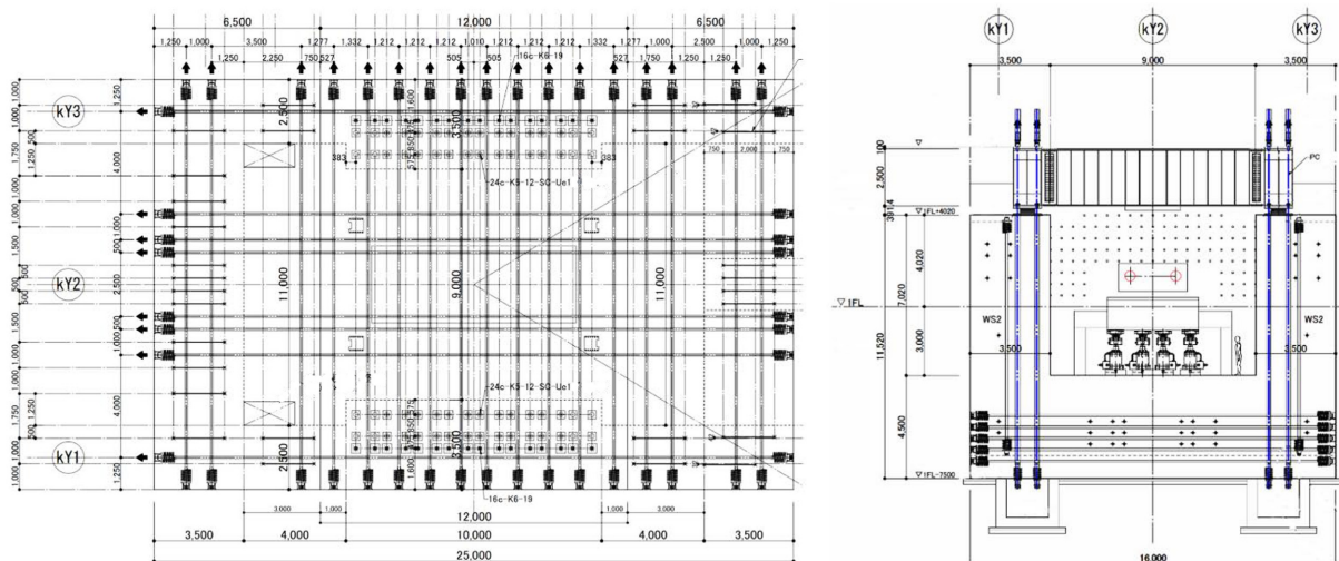
Figure 5. Plan and section of RC reaction wall with PC strand arrangement (Courtesy of Kurosawa Construction)
